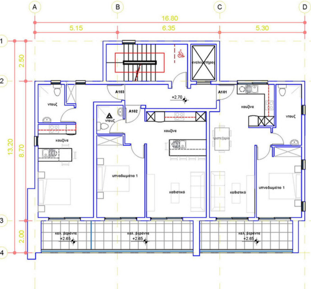
BLOCK A - First Floor
