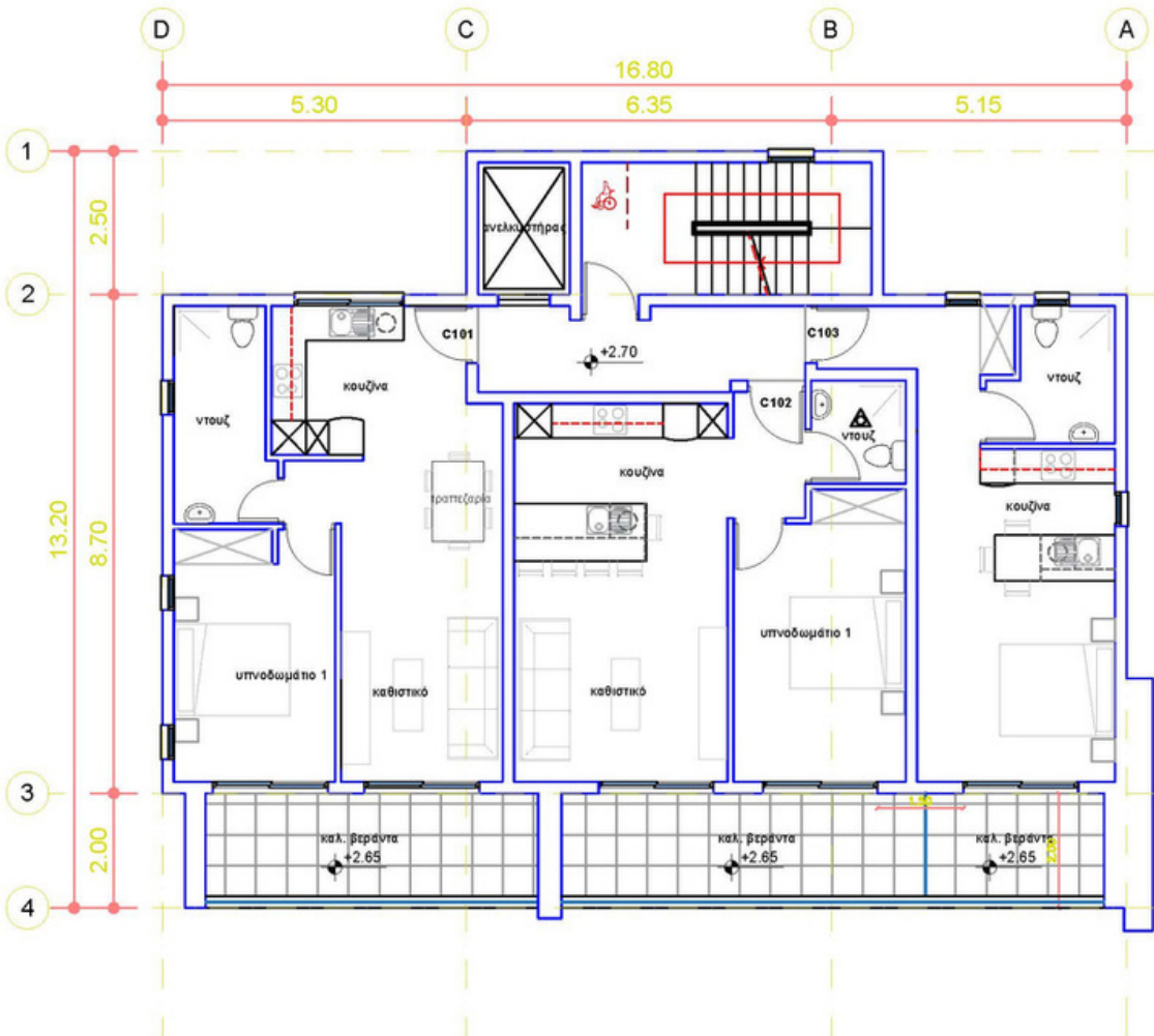
BLOCK C - First Floor
